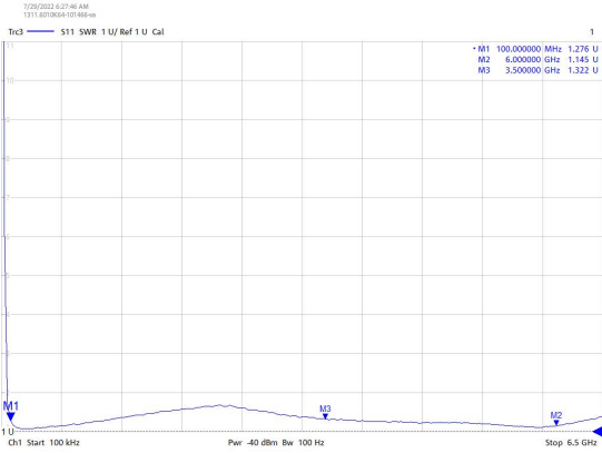
S11
