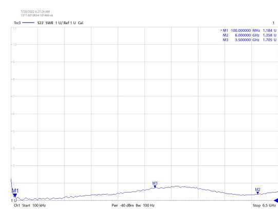
S22
